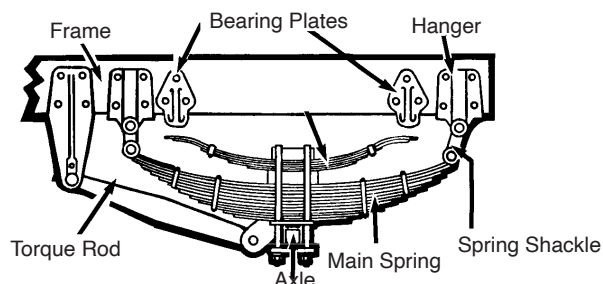
Figure 2.4 Air Suspension Parts
